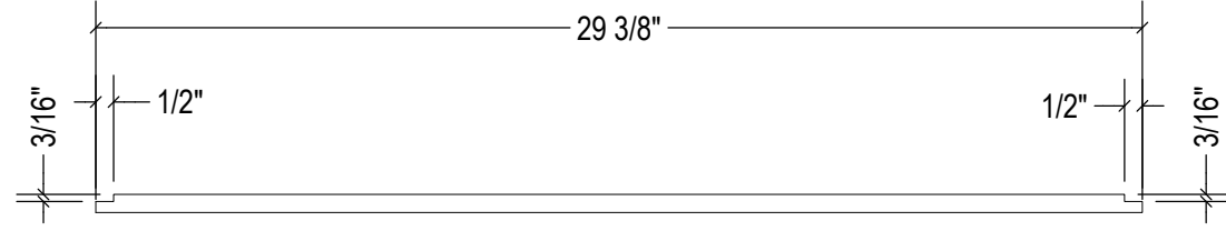
TOP SCALE 1/6
