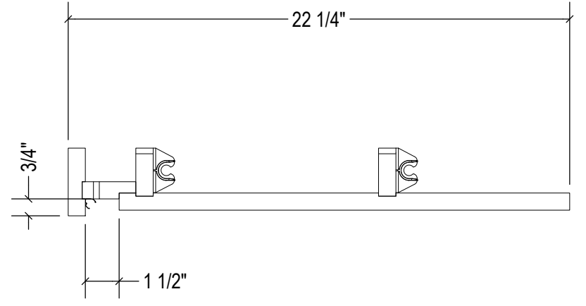
SIDE SCALE 1/6
