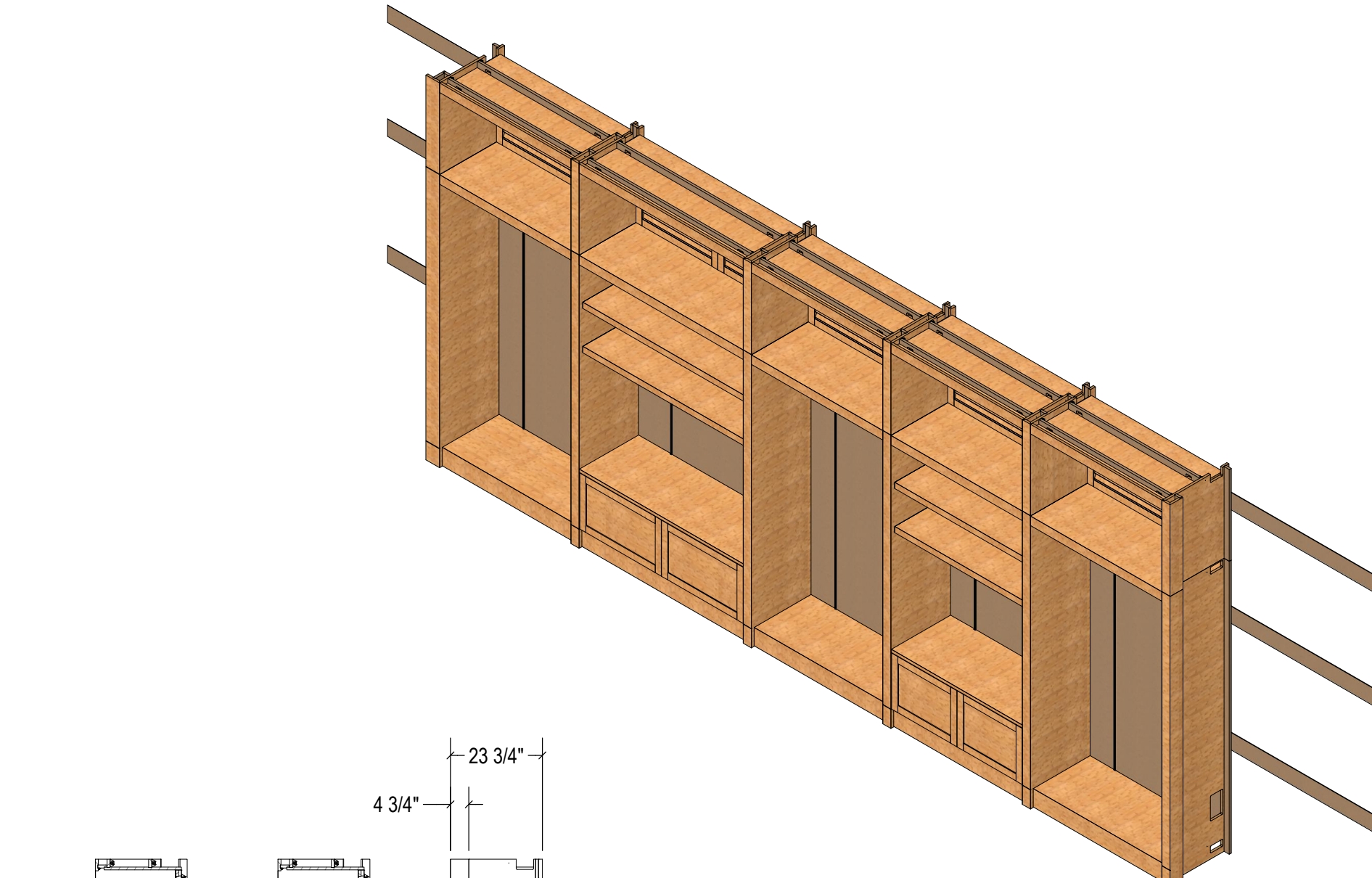
ISO SCALE 1/36
