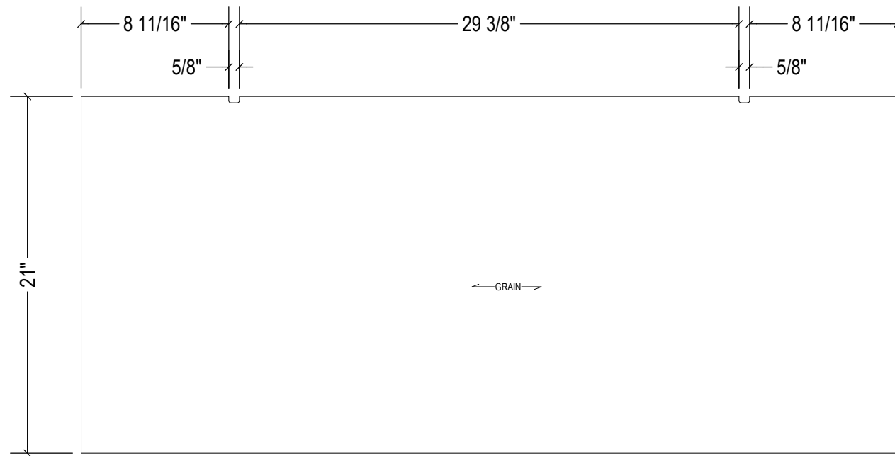
VIEW49 SCALE 1/8
