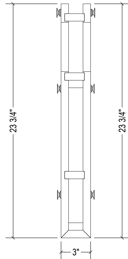
TOP SCALE 1/6
