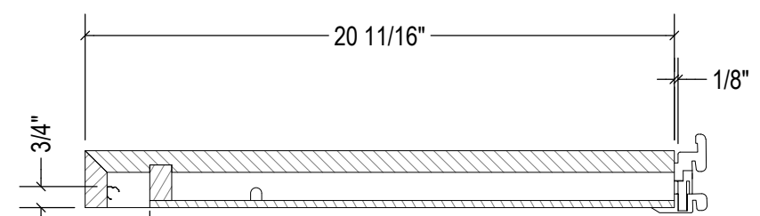
SECTION J SCALE 1/6
