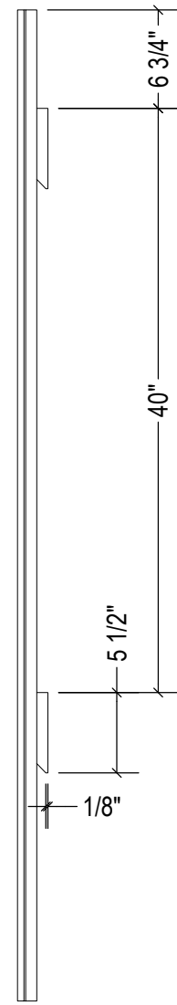
SIDE SCALE 1 / 12
