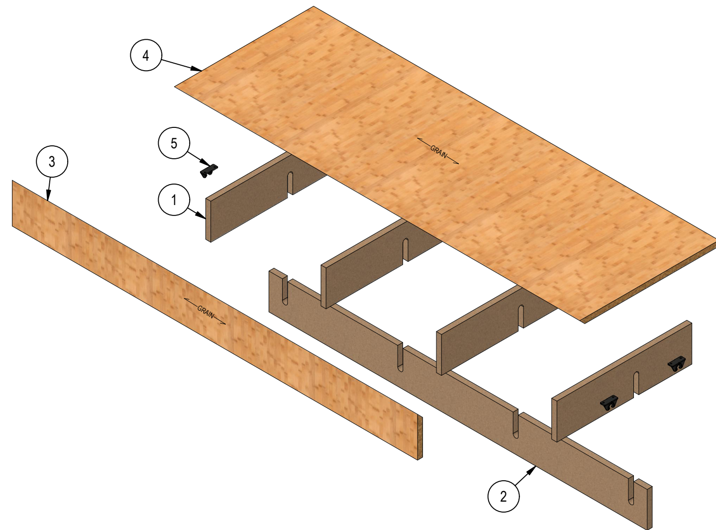
EXPLODED SCALE 1 / 10
