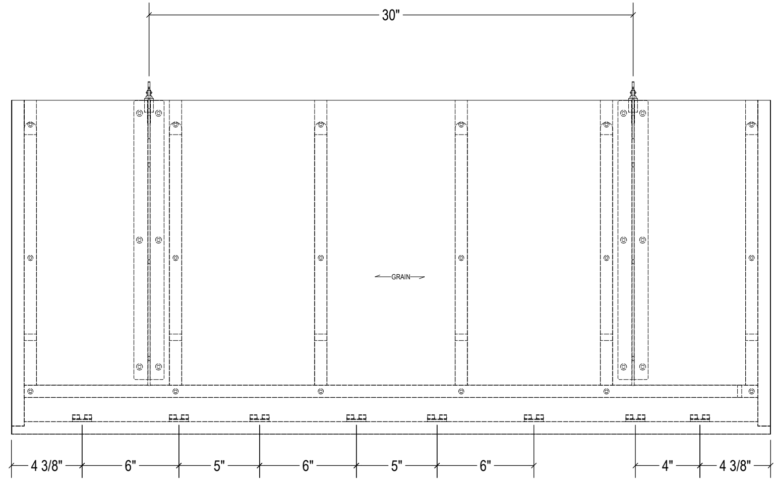
TOP SCALE 1/6
