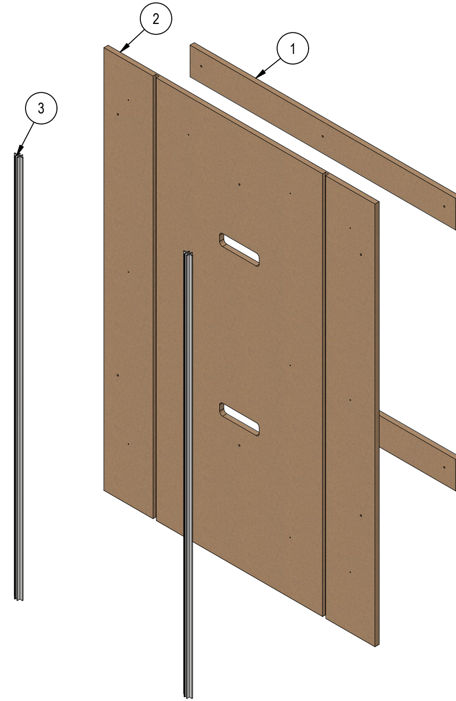
EXPLODED SCALE 1 / 12
