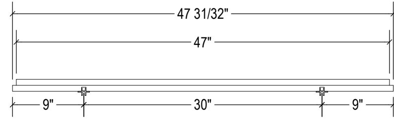
TOP SCALE 1 / 12
