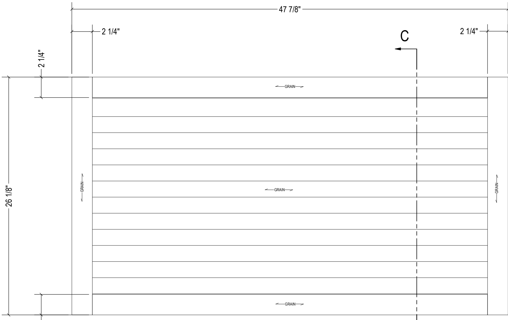
FRONT SCALE 1/6
