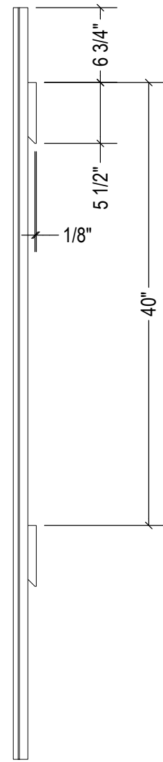
SIDE SCALE 1 / 12
