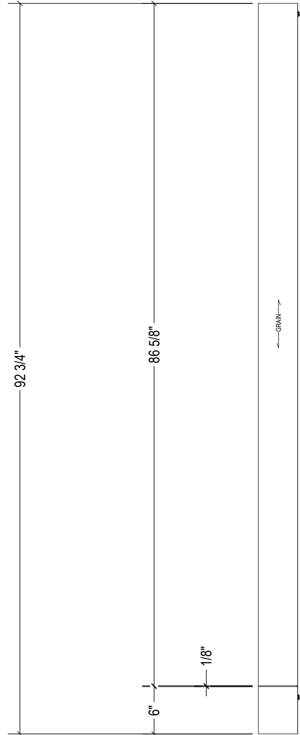
FRONT SCALE 1/12
