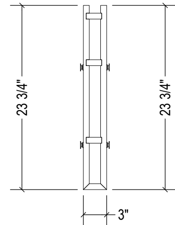
TOP SCALE 1 / 12
