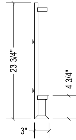
TOP SCALE 1 / 12
