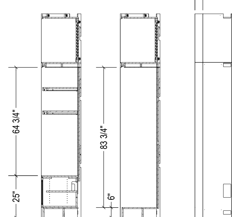
SECTION A SCALE 1/36
