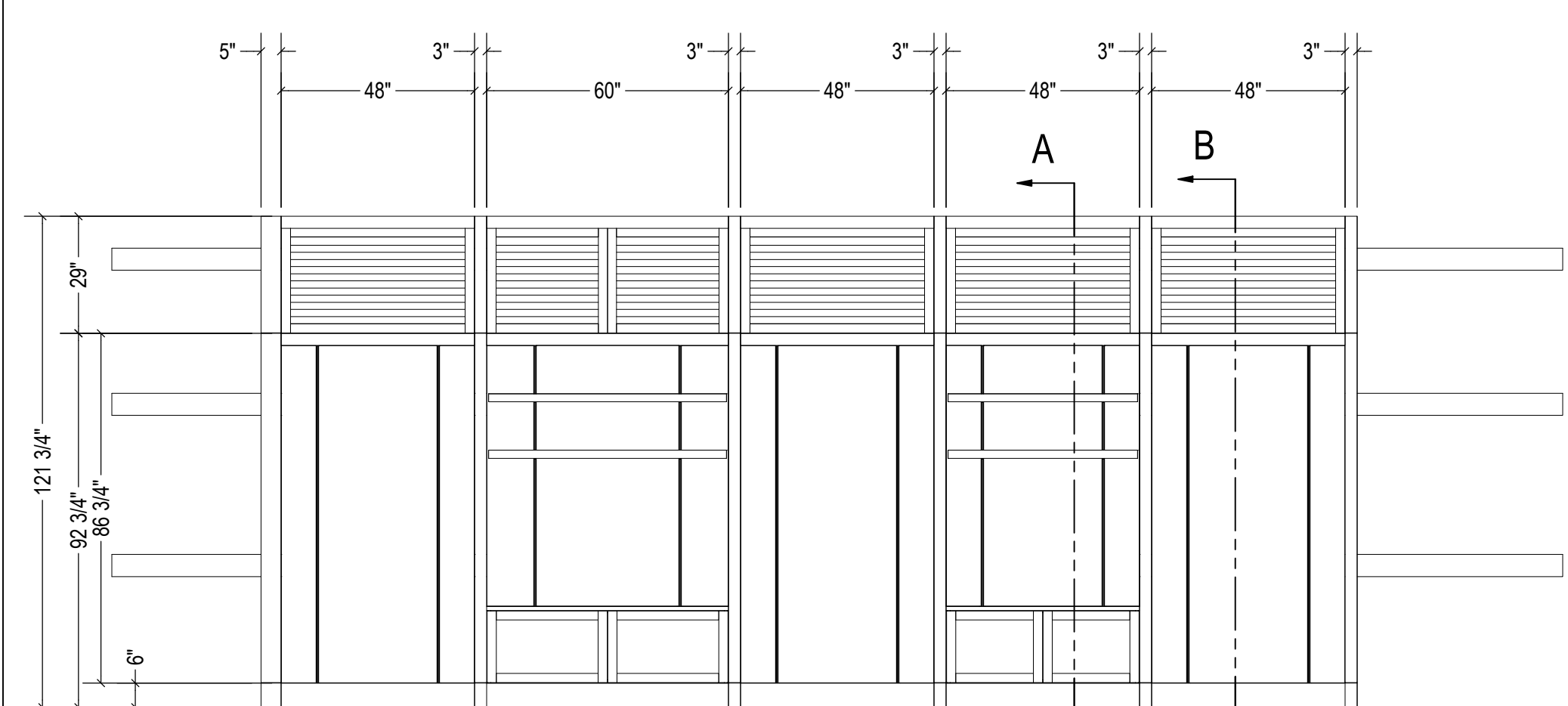
FRONT SCALE 1/36
