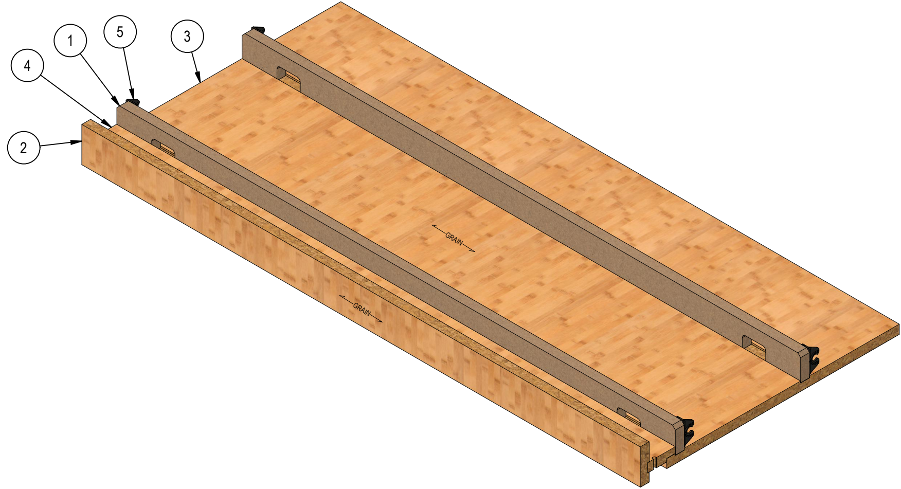
ISO SCALE 1/6
