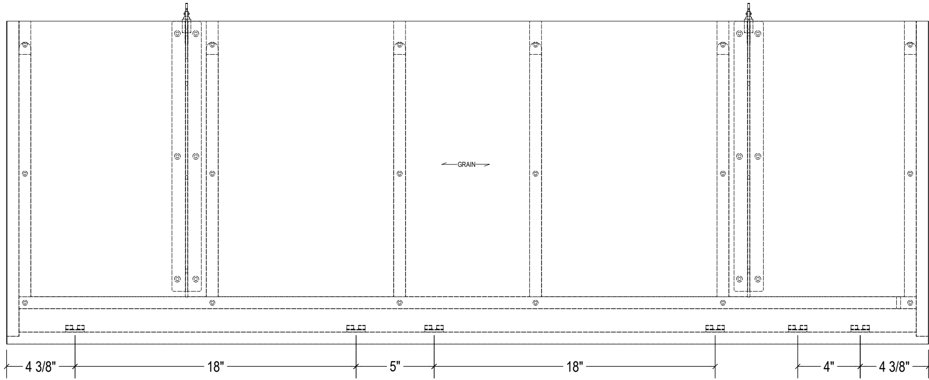
TOP SCALE 1/6
