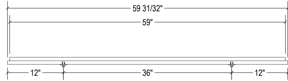
TOP SCALE 1 / 12
