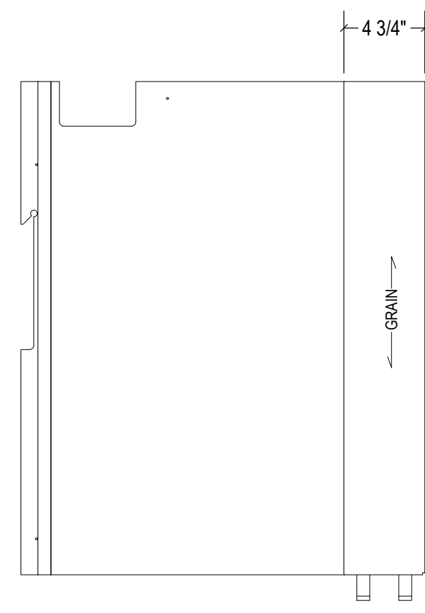
LEFT SIDE SCALE 1/8
